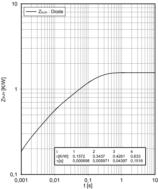
Transienter Wärmewiderstand Diode-Chopper transient thermal impedance Diode-Chopper Z_{thJH} = f(t)
