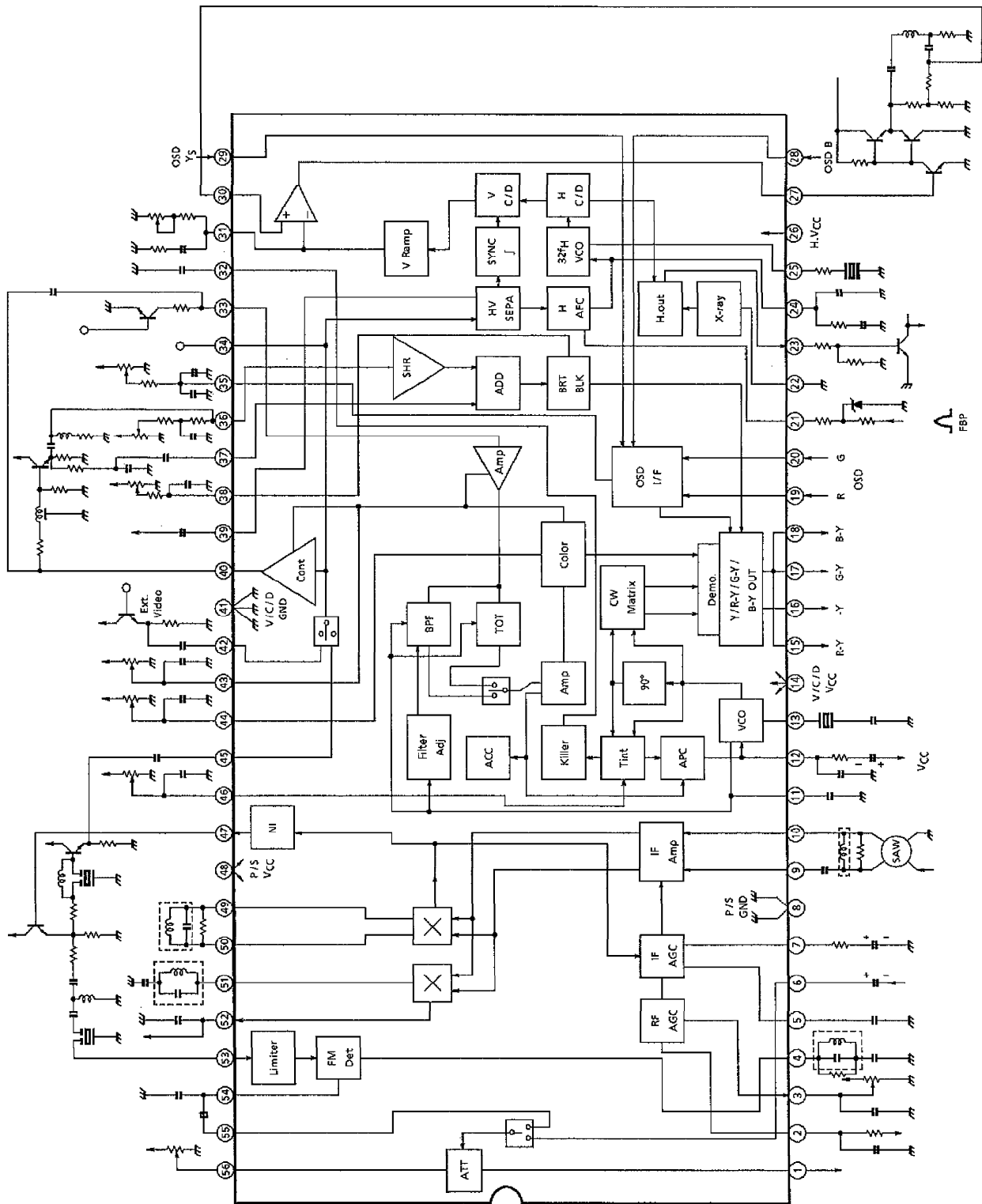
BLOCK DIAGRAM
