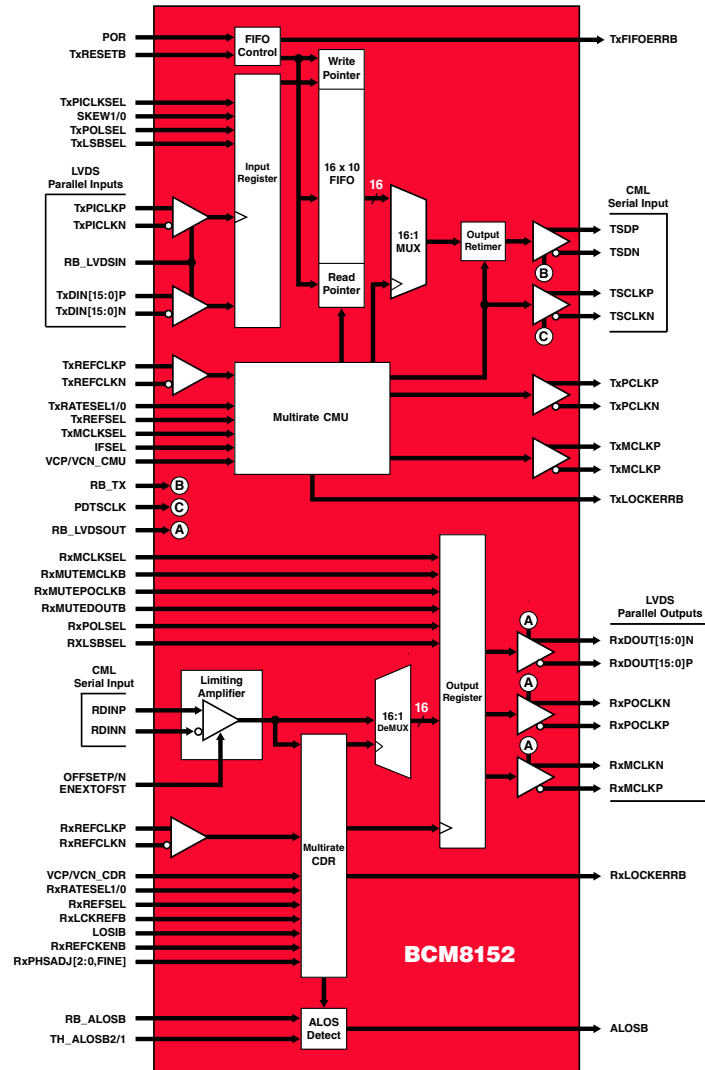
BCM8152 Block Diagram
