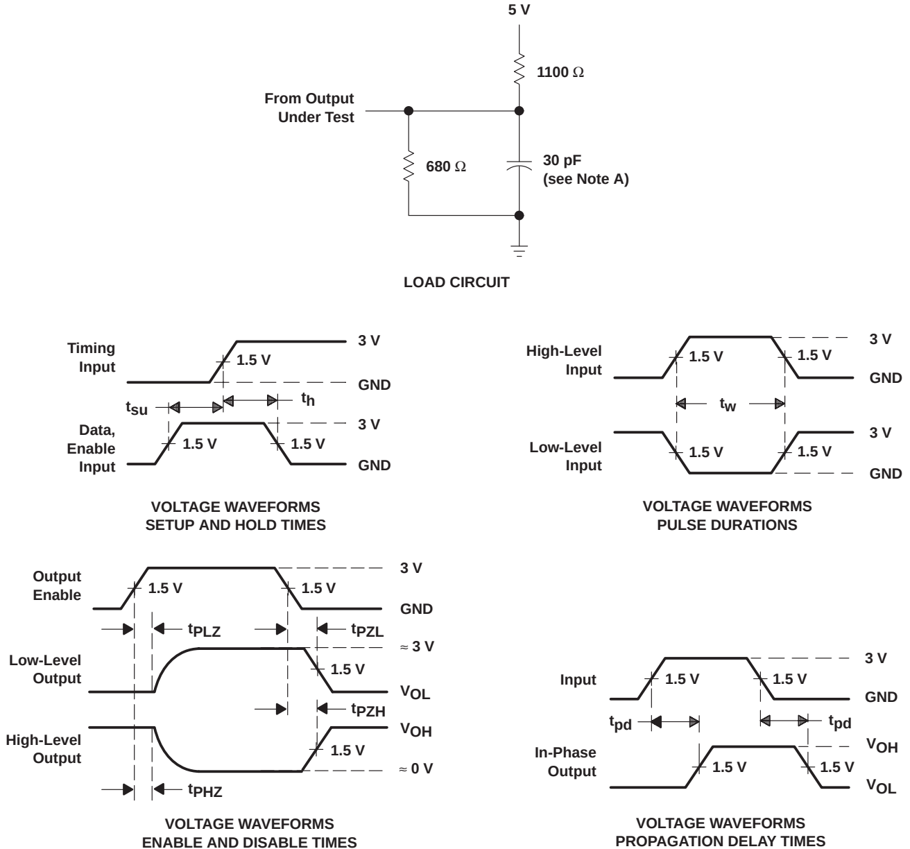
Figure 13. Load Circuit and Voltage Waveforms
