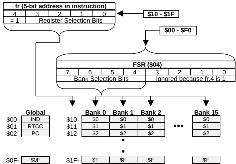
Figure 27 - SX48/52 General-Purpose Register addressing (direct)
