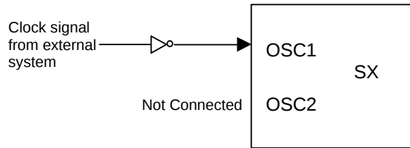
Figure 39 - SX with External System Clock
