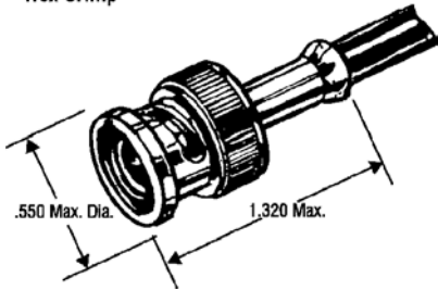
Hex Crimp
