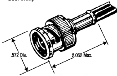
Dual Crimp
