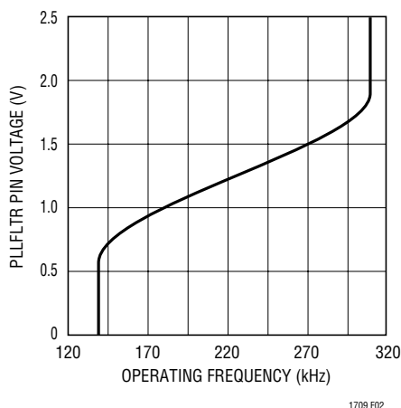
Figure 2. Operating Frequency vs V_{\text{PLLFLTR}}
