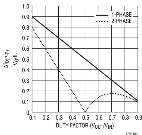
Figure 3. Normalized Output Ripple Current vs Duty Factor [ I_{\text{RMS}} \approx 0.3 (\Delta I_{\text{O(P-P)}) ]
