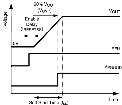
Figure 8-4. Soft-Start Timing
