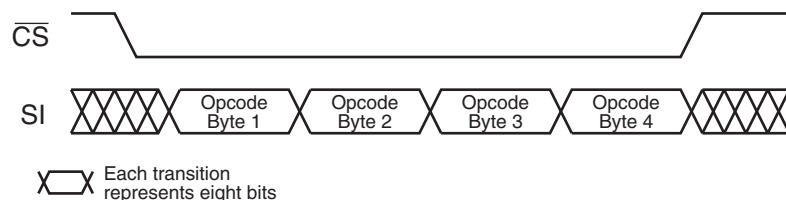
Figure 7-1. Chip Erase
