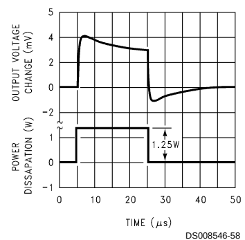
Thermal Response
