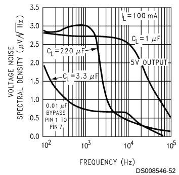
LP2951 Output Noise
