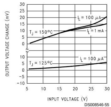
Line Regulation
