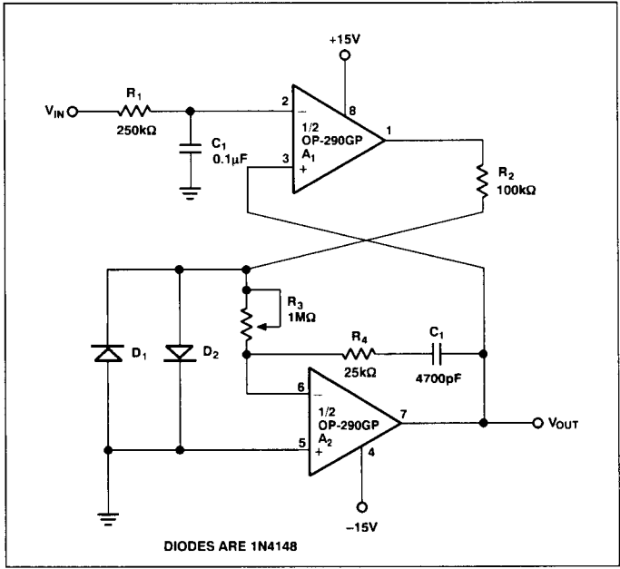
FIGURE 3: Variable Slew Rate Filter
