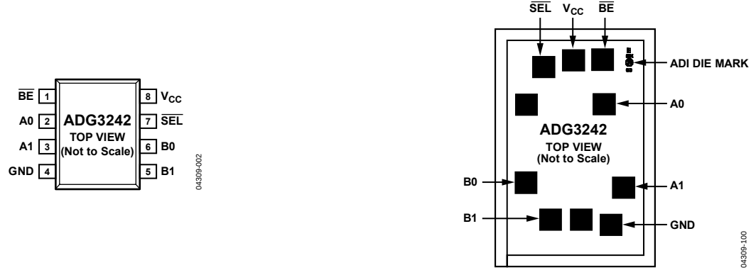
Figure 2. Pin Configuration Figure 3. Die Pad Configuration (Die size: 550 μm × 820 μm)
