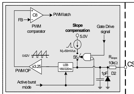
Figure 9 Slope compensation
