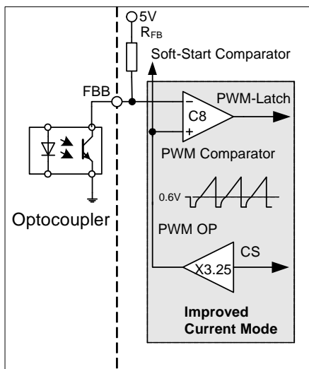
Figure 8 PWM Controlling
