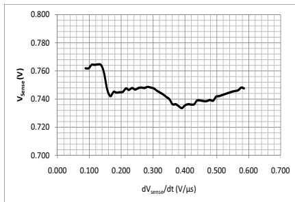
Figure 22 Overcurrent Shutdown
