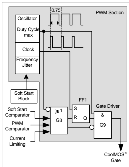
Figure 15 PWM Section Block
