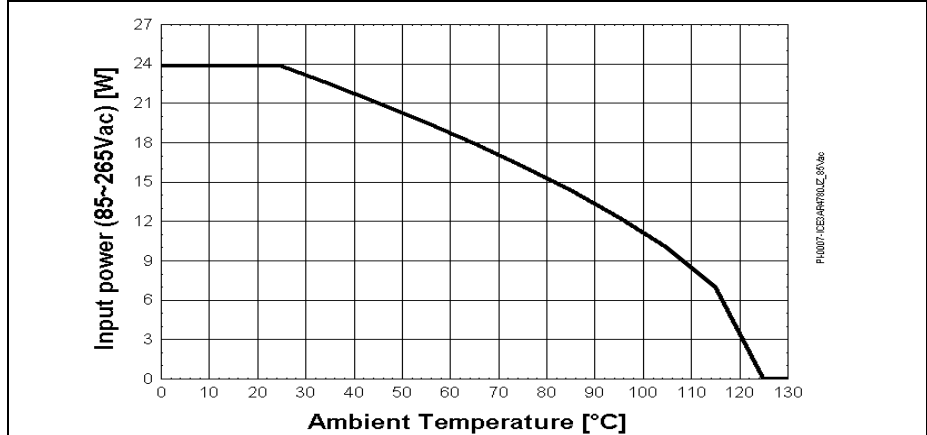
Figure 38 Input power curve V_{in}=85\sim 265V_{ac} ; P_{in}=f(T_a)
