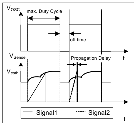
Figure 21 Dynamic Voltage Threshold V_{csth}
