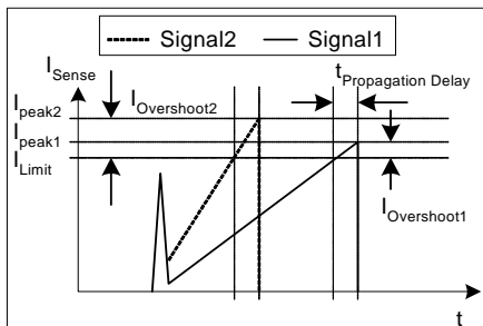
Figure 20 Current Limiting
