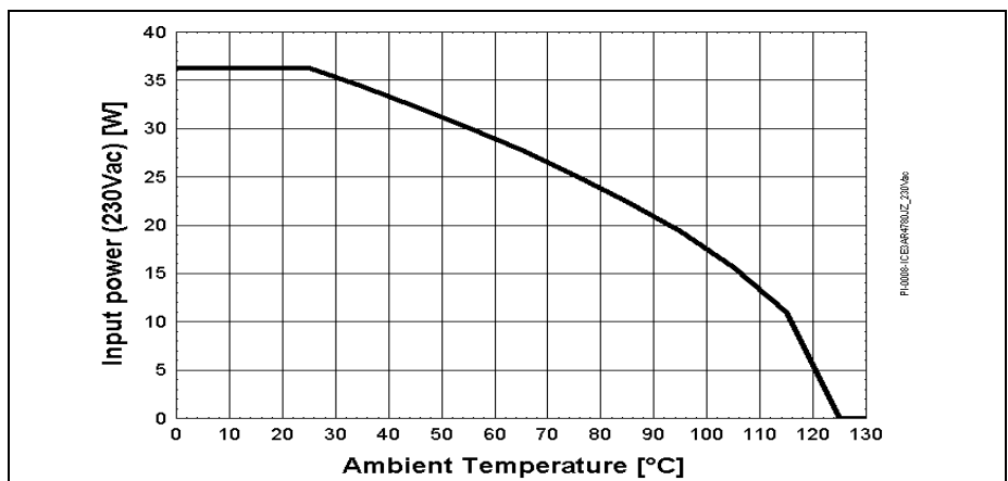
Figure 39 Input power curve V_{in}=230V_{ac}\pm 15\% ; P_{in}=f(T_a)
