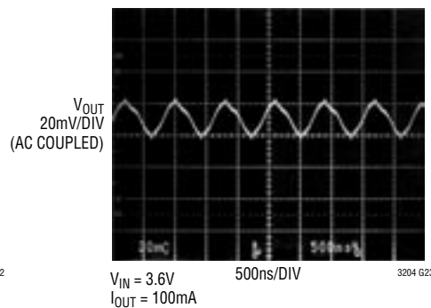
Output Ripple
