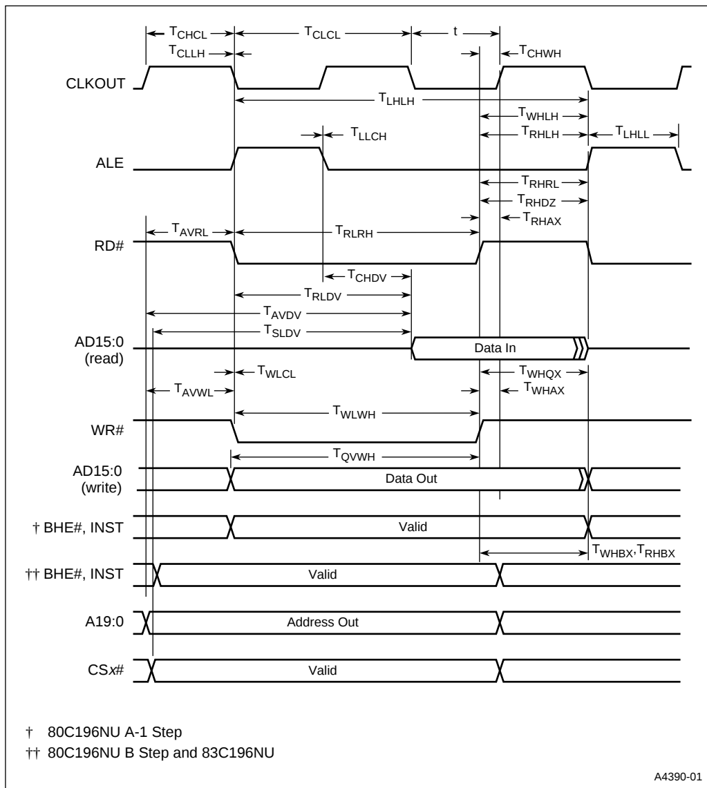
Figure 9. System Bus Timings, Demultiplexed Bus Mode
