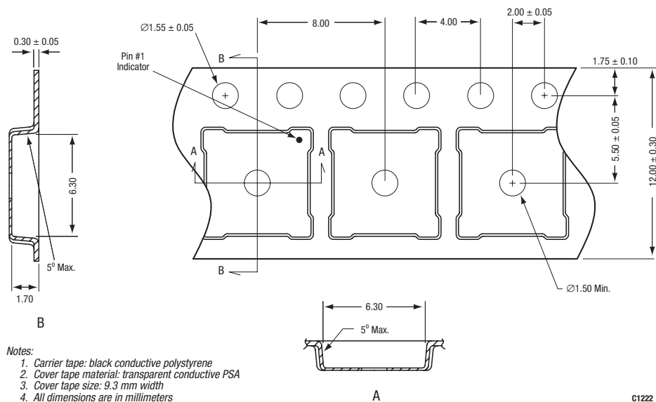
Figure 8. SKY73022-11 Tape and Reel Dimensions
