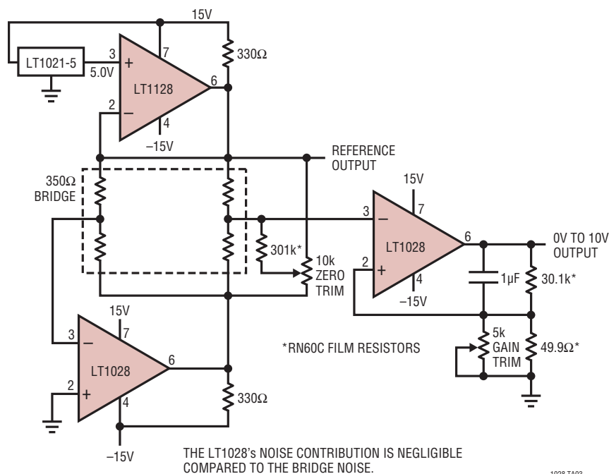
Strain Gauge Signal Conditioner with Bridge Excitation
