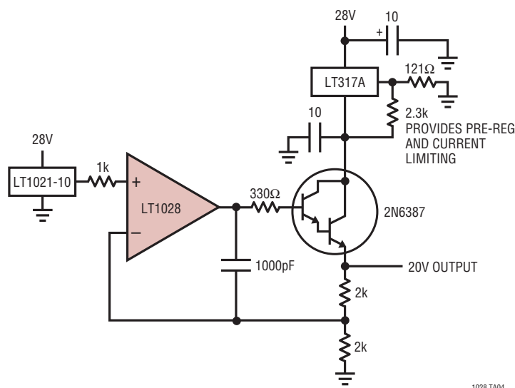
Low Noise Voltage Regulator
