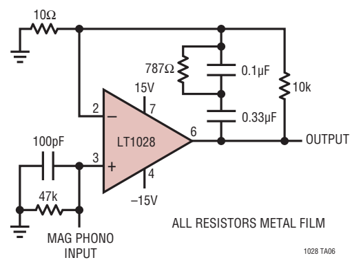
Phono Preamplifier
