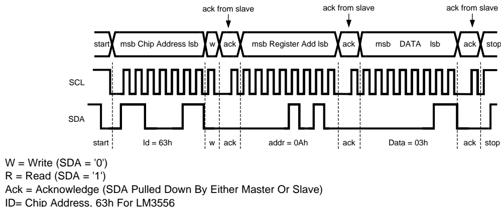
Figure 31. Write Cycle
