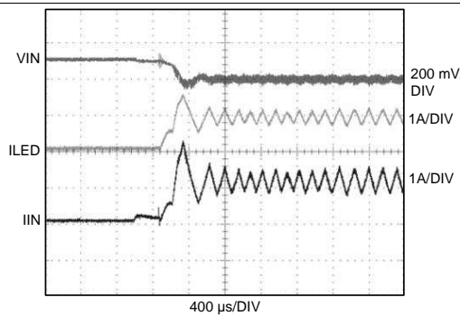
Figure 23. Input Voltage Flash Monitor, Up and Down Mode
