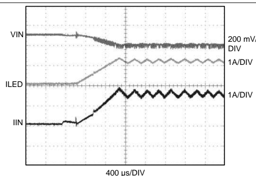
Figure 21. Input Voltage Flash Monitor Down Mode With Default Settings
