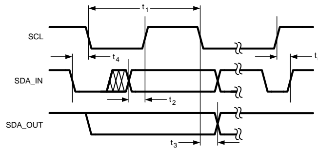
Figure 1. I²C-Compatible Timing Diagram
