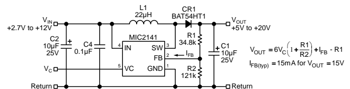
Figure 2. Gain-Boost Configuration
