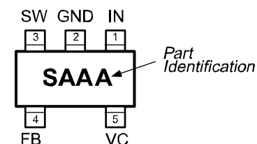
5-Pin SOT23 (BM5)
