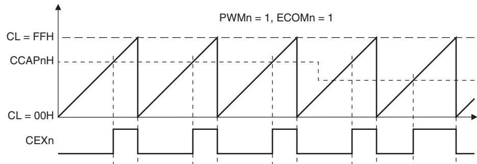
Figure 15-8. PCA PWM Waveform
