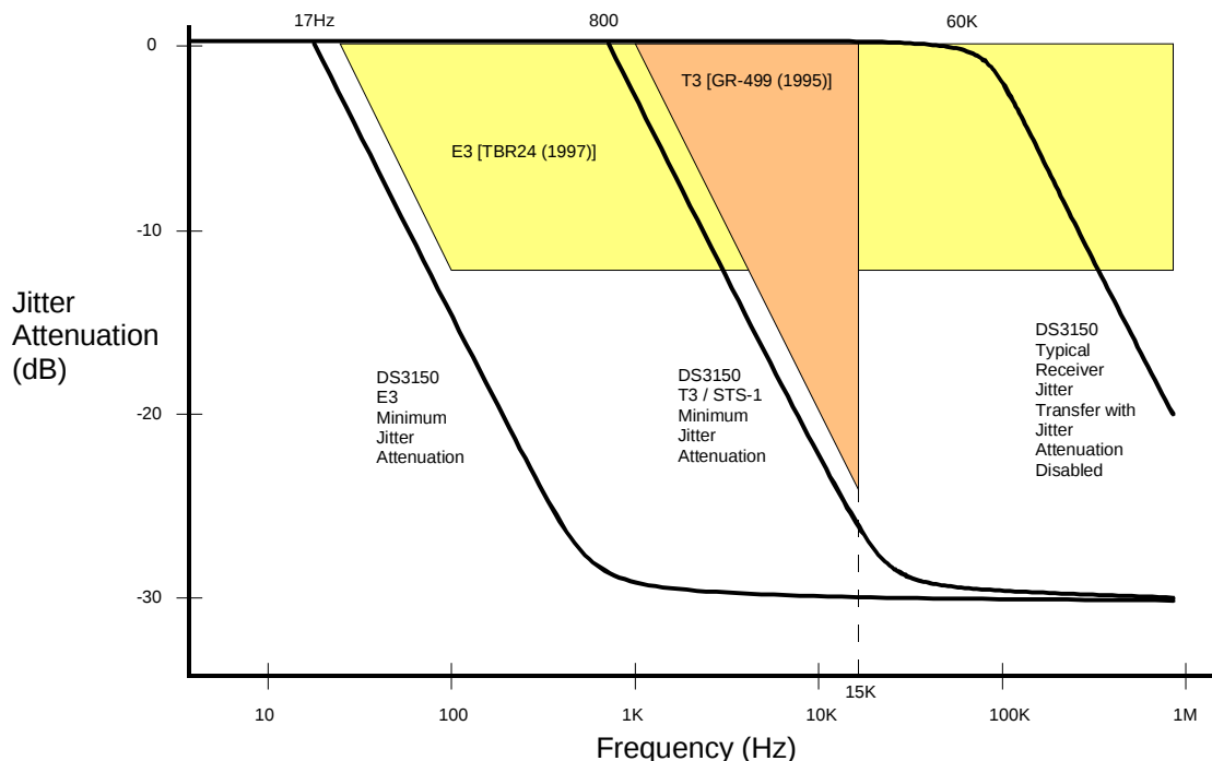
DS3150 JITTER ATTENUATION / JITTER TRANSFER Figure 1H
