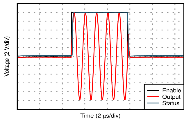
Figure 22. Enable Response
