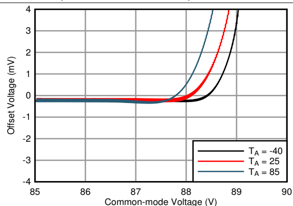
Figure 8. Offset Voltage vs Common-Mode Voltage (High V_{CM} )
