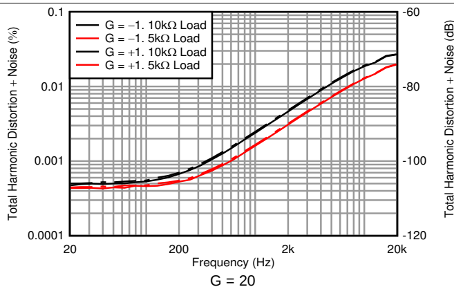
Figure 47. THD+N Ratio vs Frequency
