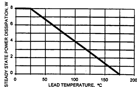
Fig. 4. STEADY STATE POWER DERATING
