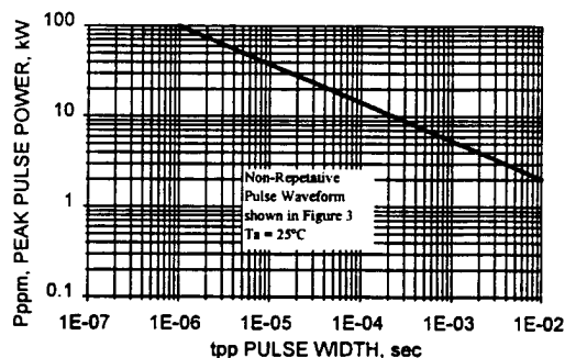
Fig. 2. PEAK PULSE POWER RATING CURVE
