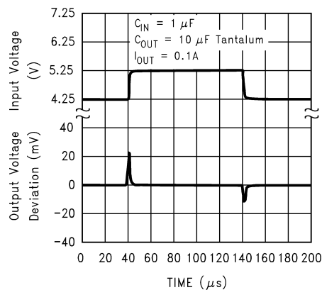
LM1117-2.85 Line Transient Response
