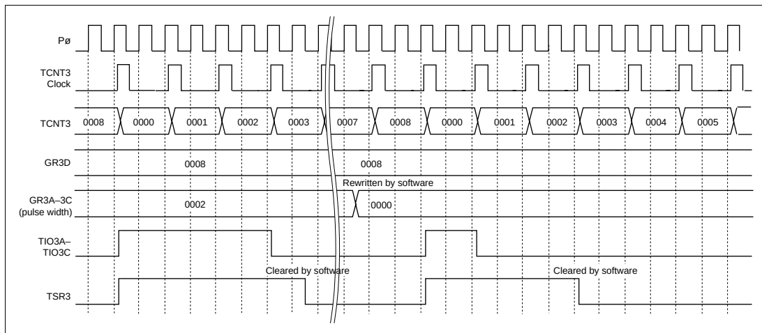
Figure 10.23 Channel 3 to 5 PWM Mode Operation
