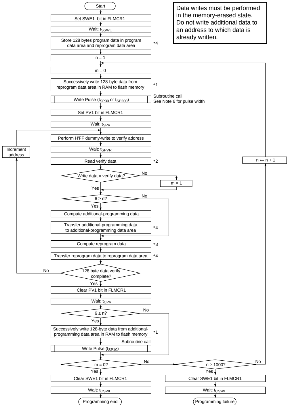
Figure 20.13 Program/Program-Verify Flowchart (1)
