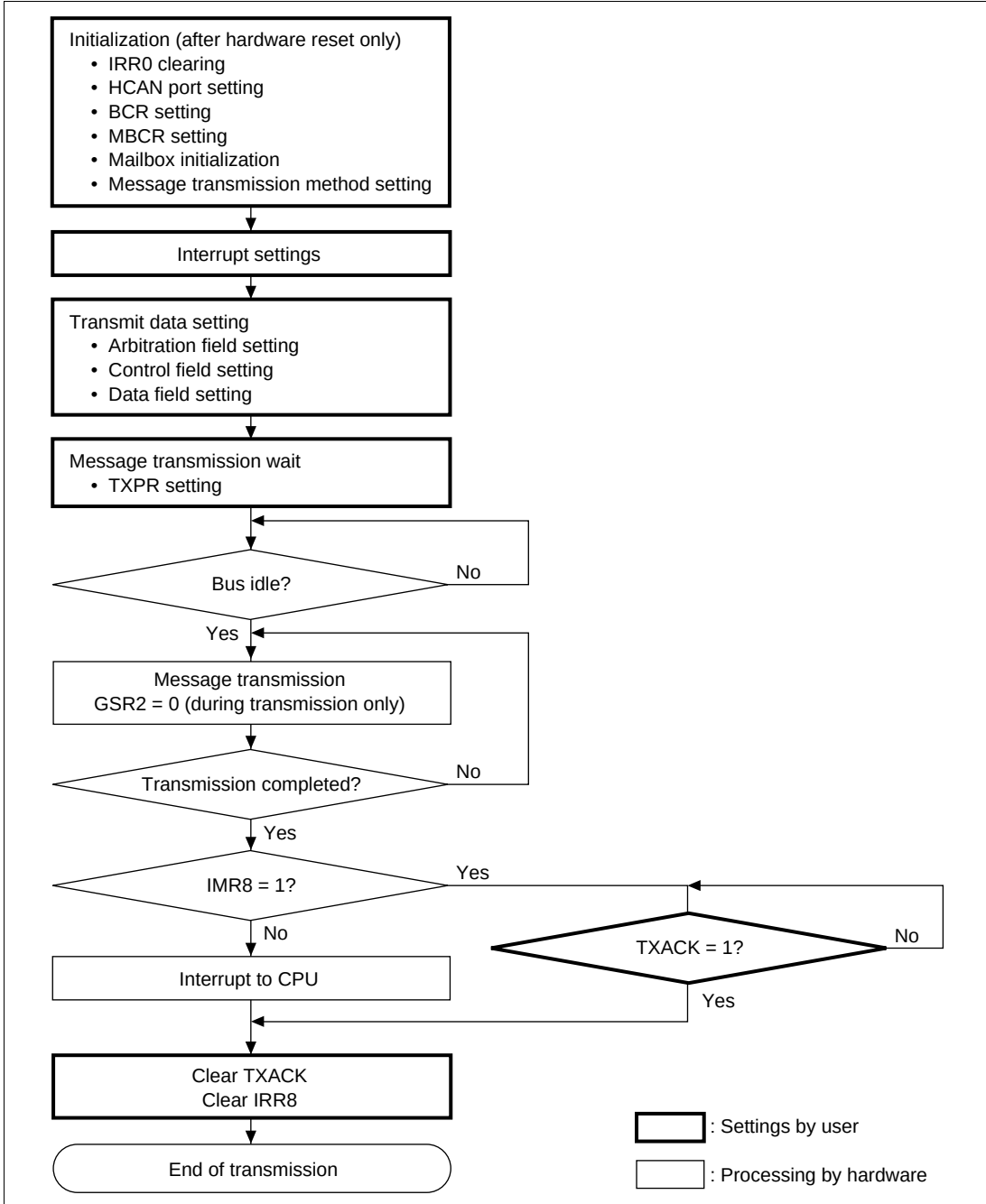
Figure 15.7 Transmission Flowchart
