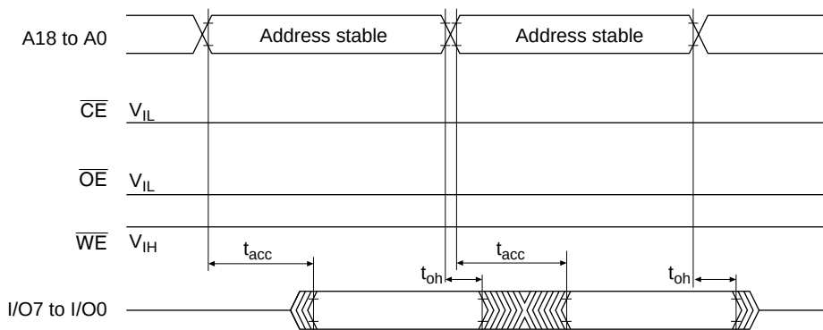
Figure 20.23 \overline{\text{CE}} and \overline{\text{OE}} Enable State Read Timing Waveforms
