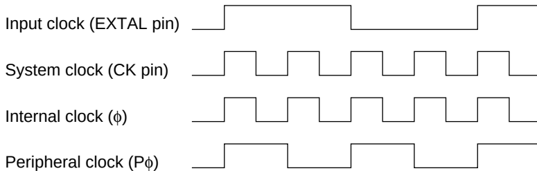
Figure 4.2 Input Clock and System Clock
