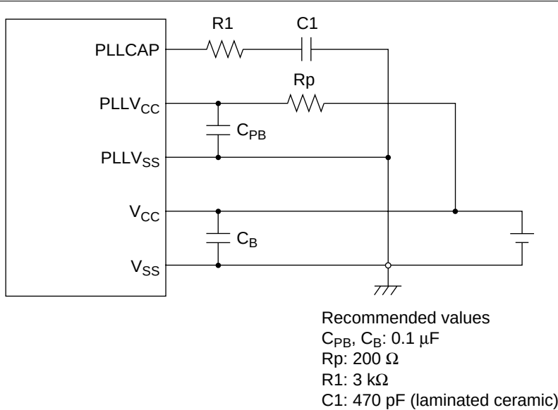
Figure 4.7 Points for Caution in PLL Power Supply Connection
