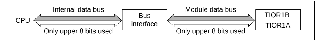
Figure 10.49 Byte Read/Write Access to TIOR1B
