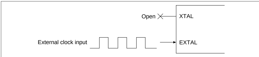
Figure 4.5 External Clock Input Method (Example)
