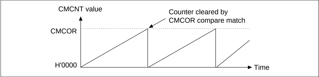
Figure 13.2 Counter Operation
