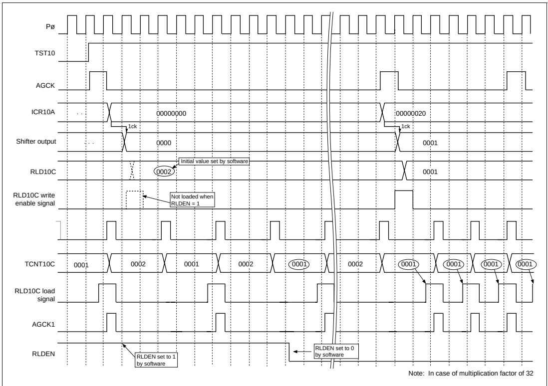
Figure 10.30 TCNT10C Operation
