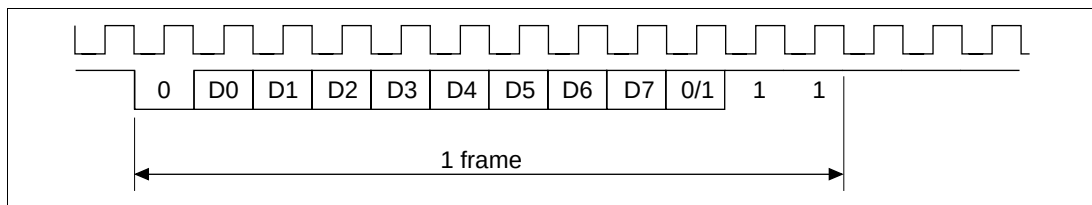
Figure 14.3 Output Clock and Communication Data Phase Relationship (Asynchronous Mode)
