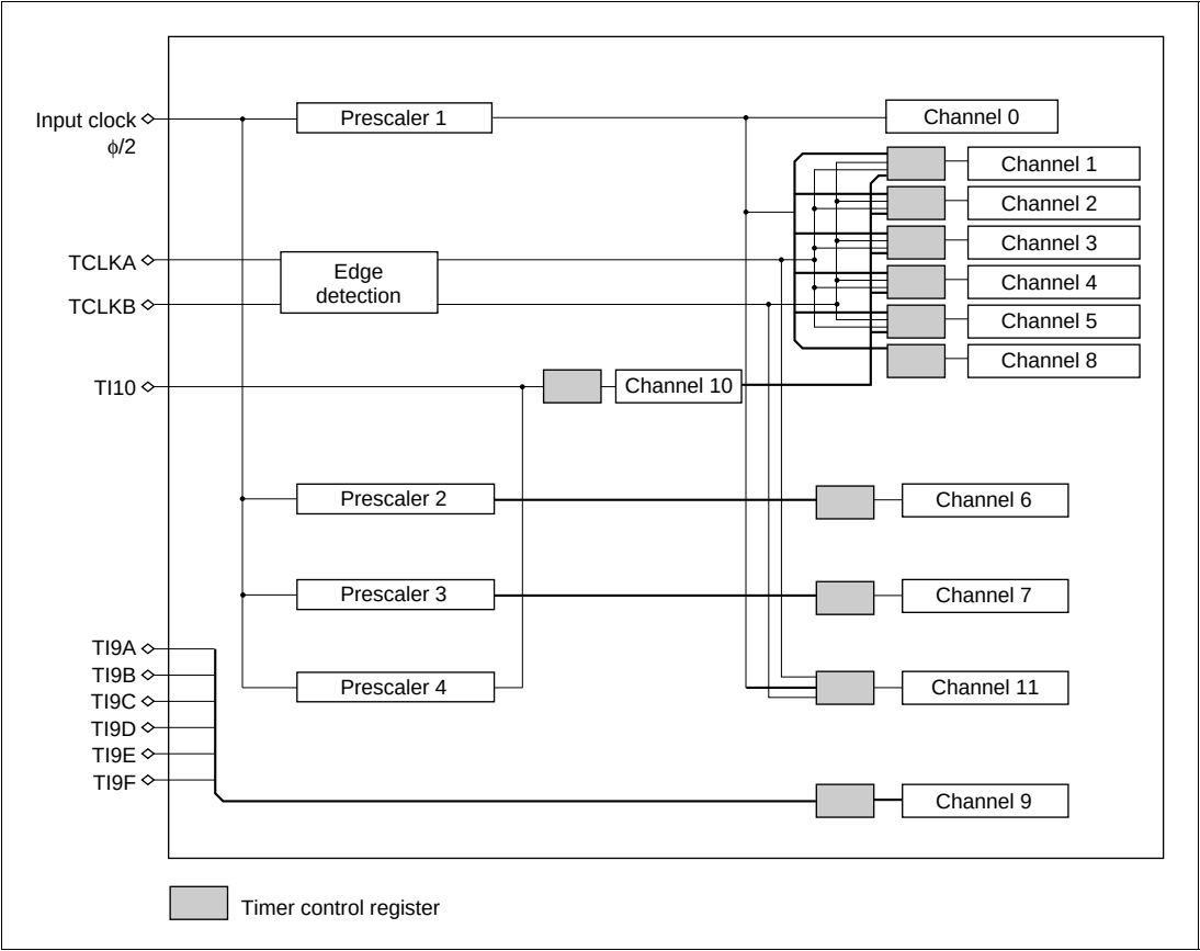
Figure 10.12 Prescaler Diagram
