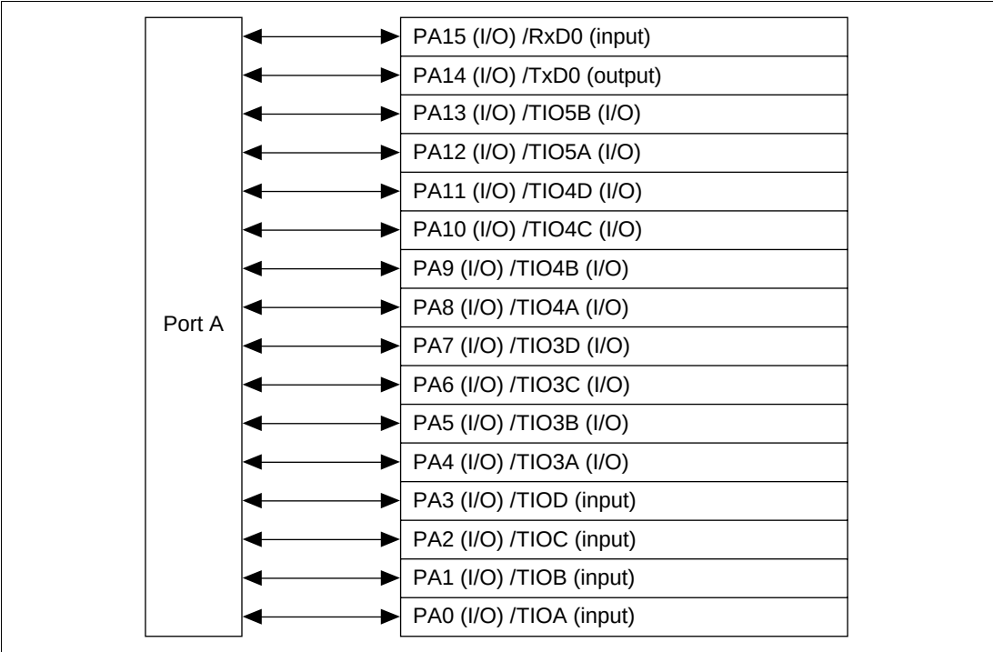
Figure 19.1 Port A
