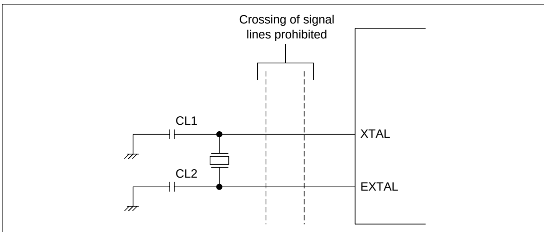
Figure 4.6 Precautions for Oscillator Circuit System Board Design
