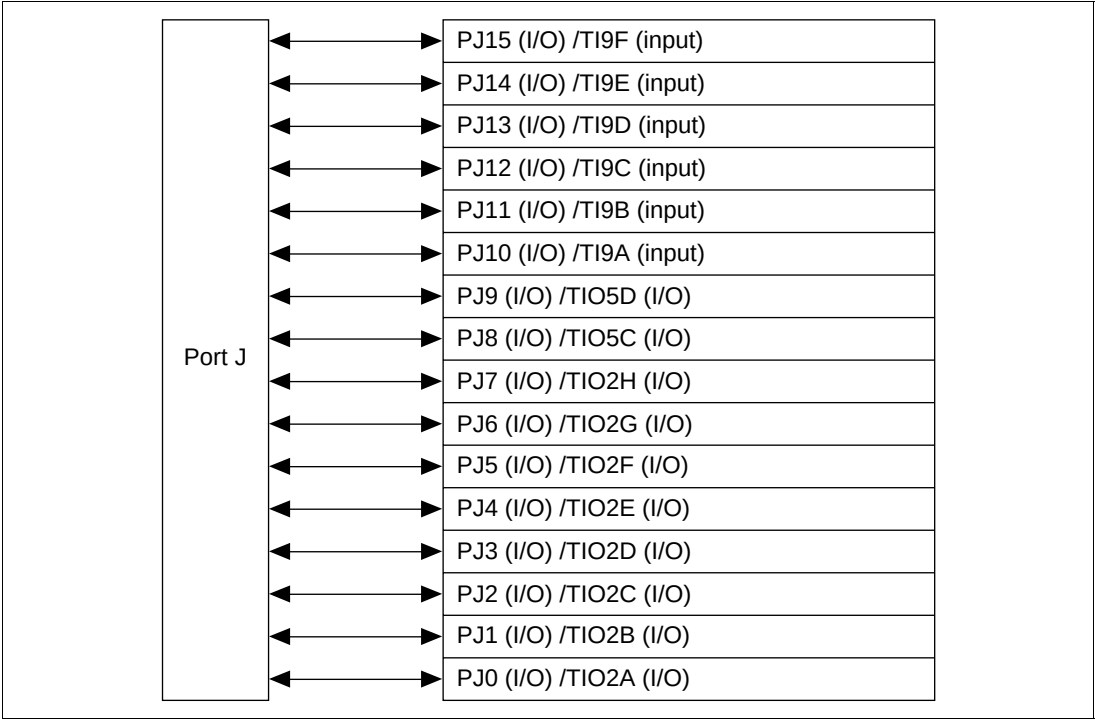
Figure 19.9 Port J
