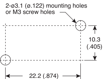
Mounting Holes
