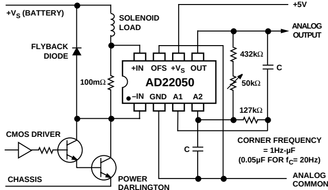
Figure 11. Illustration of Two-Pole Low-Pass Filtering
