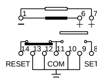
2 coil latching
