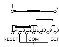
1 coil latching
