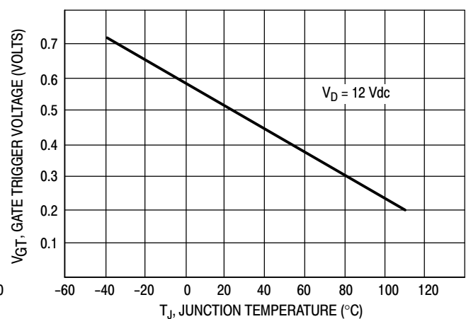
Figure 4. Gate Voltage
