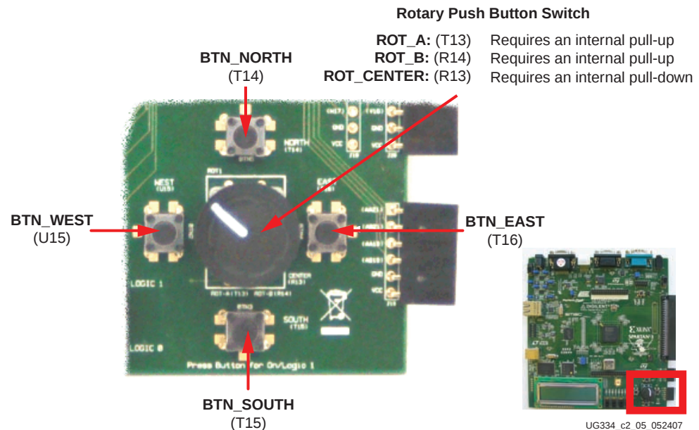
Figure 2-5: Four Push-Button Switches Surround the Rotary Push-Button Switch
