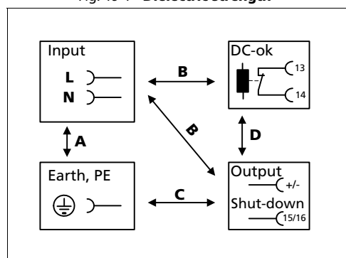
Fig. 19-1 Dielectric strength
