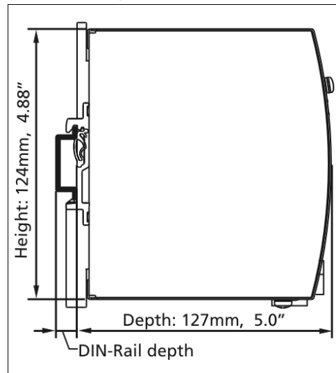
Fig. 23-2 Side view
