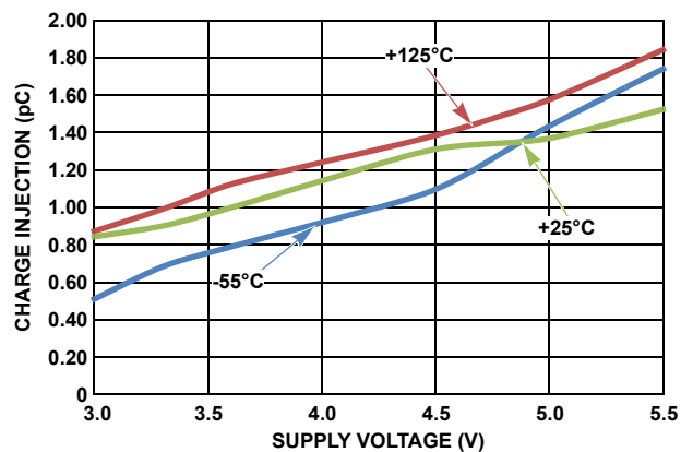
FIGURE 28. CHARGE INJECTION
