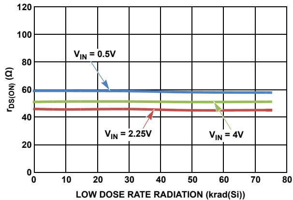
FIGURE 29. r_{DS(ON)} ( V^+ = 4.5V ), BIASED
