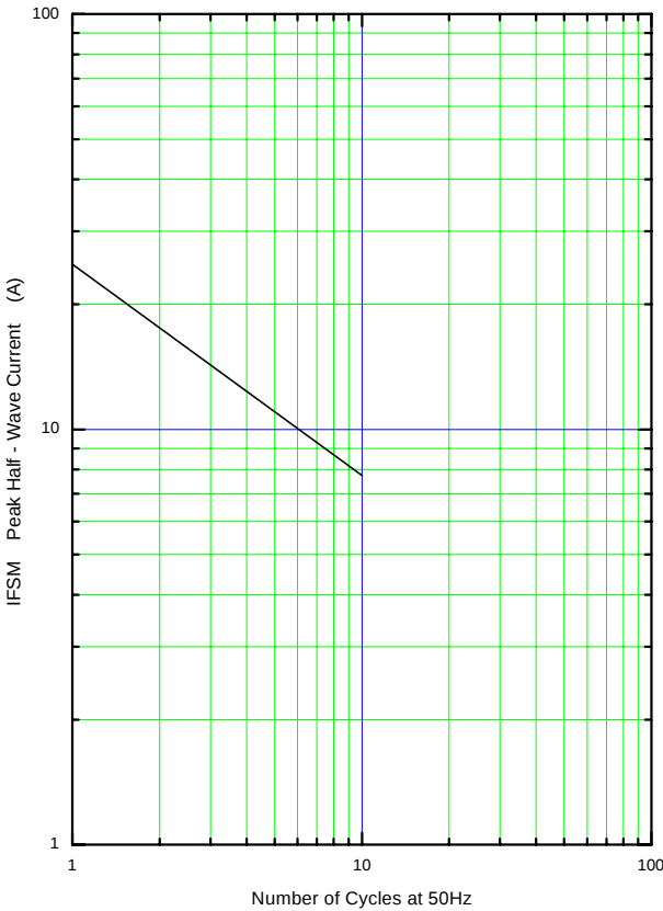
Surge Capability
