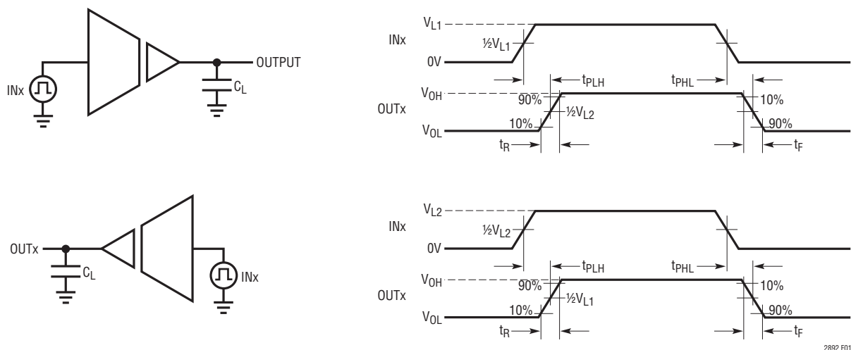
Figure 1. Logic Timing Measurements
