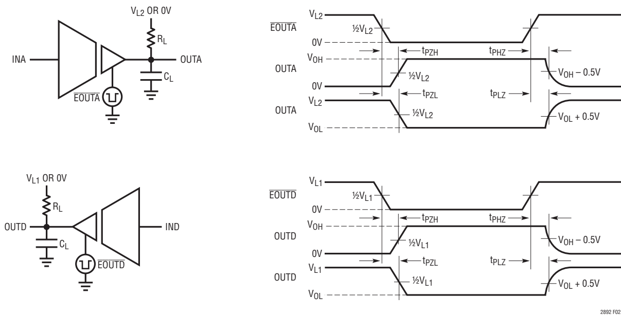
Figure 2. Logic Enable/Disable Time
