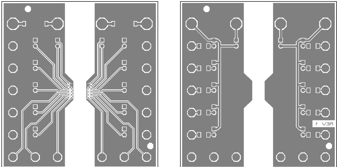
Figure 22a. LTM2892-S Demo Board Layout (DC1957A)
