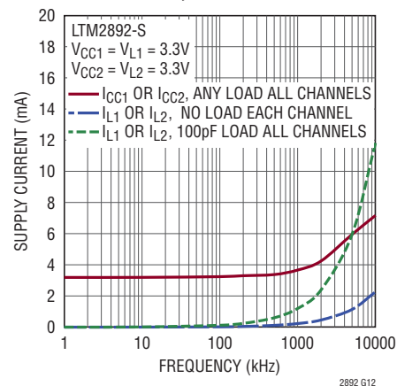
Supply Current vs Data Rate, All Channels
