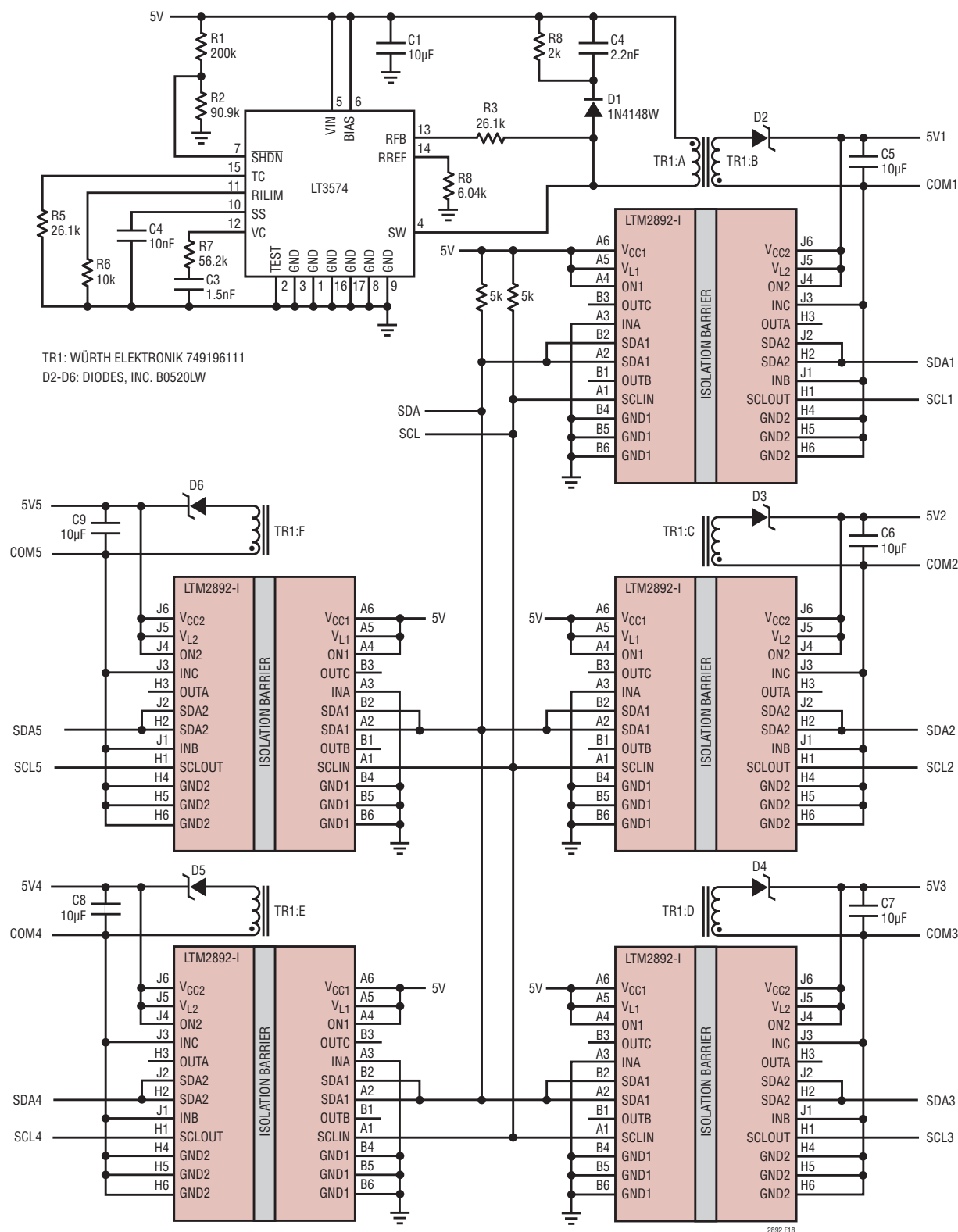
Figure 26. Parallel Multi-Zone Isolated I²C Interface
