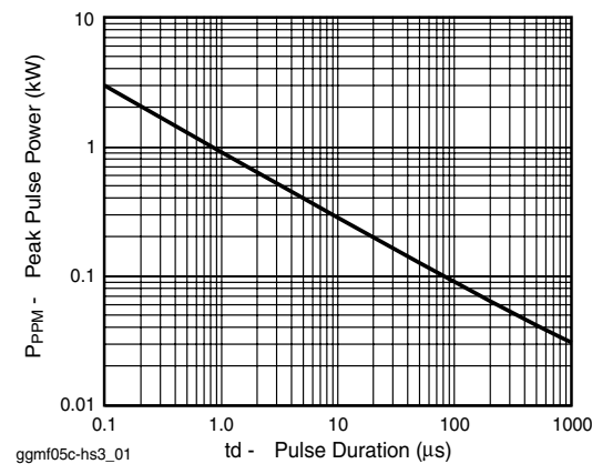
Figure 1. Non-Repetitive Peak Pulse Power vs. Pulse Time
