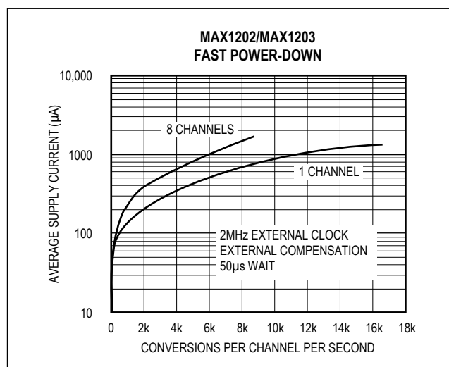
Figure 14b. MAX1202/MAX1203 Supply Current vs. Sample Rate/Second, FASTPD, 2MHz Clock
