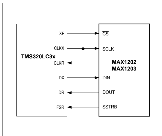
Figure 19. MAX1202/MAX1203-to-TMS320 Serial Interface
