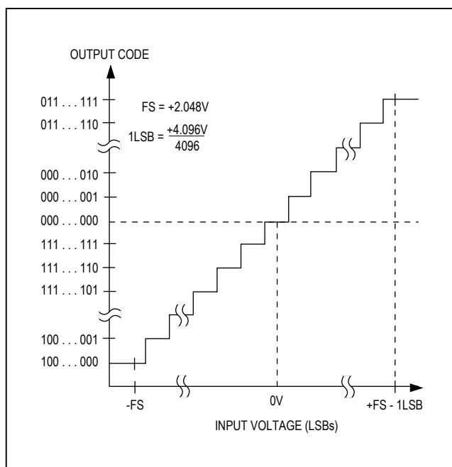
Figure 16. Bipolar Transfer Function, \pm 4.096\text{V}/2 = Full Scale
