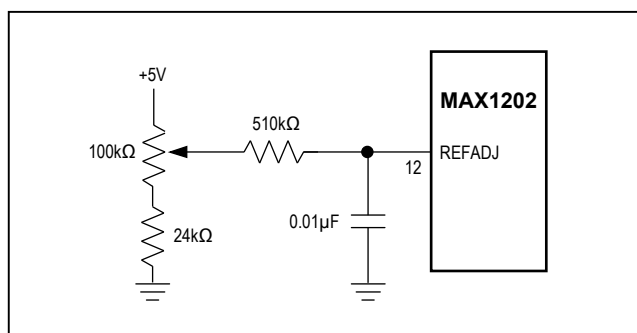
Figure 17. MAX1202 Reference-Adjust Circuit
