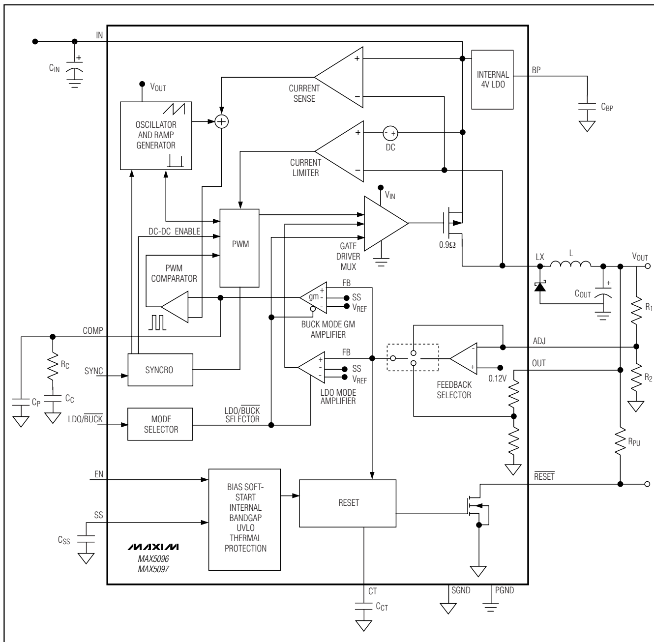
Figure 1. Simplified Diagram
