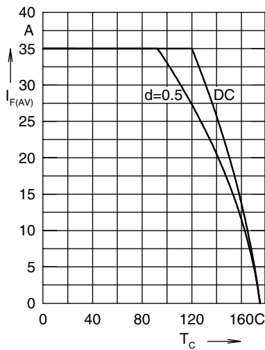
Fig. 4 Avg: forward current I_{F(AV)} vs: case temperature T_C
