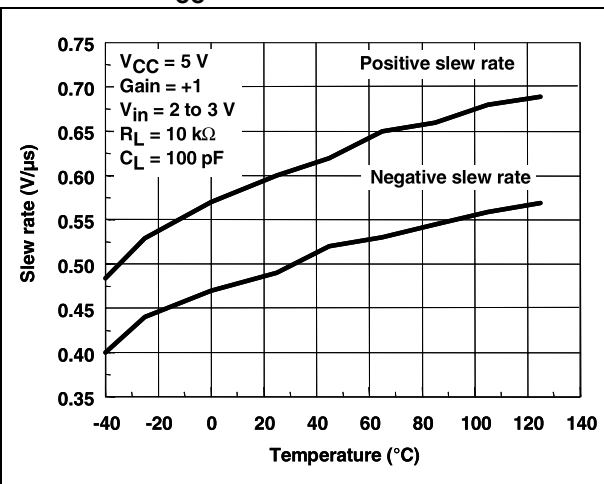
Figure 32. Slew rate vs. temperature at V_{CC} = 5\text{ V}
