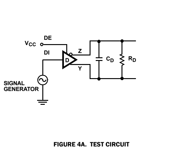
FIGURE 4A. TEST CIRCUIT
