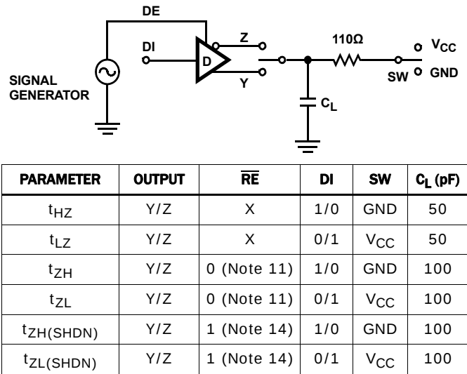
FIGURE 4. DRIVER PROPAGATION DELAY AND DIFFERENTIAL TRANSITION TIMES
