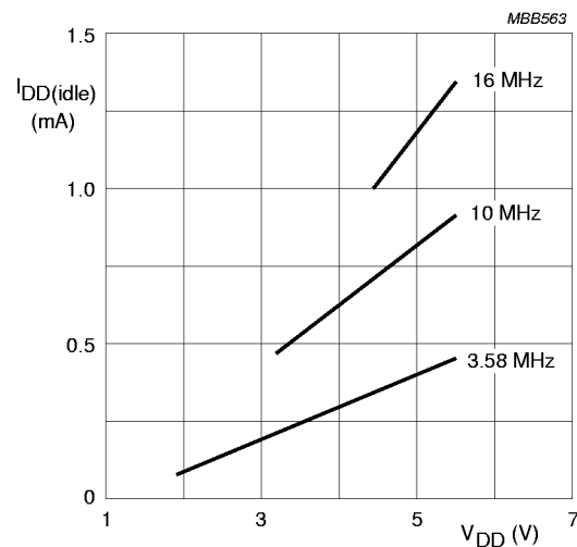
Fig.6 Typical supply current in Idle mode ( I_{DD(idle)} ) as a function of operating supply voltage ( V_{DD} ).
