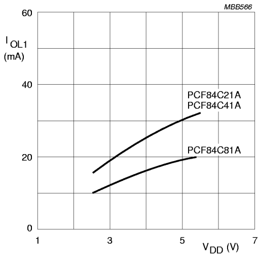
Fig.10 Typical LOW level output sink current for Port 1 ( I_{OL1} ) as a function of operating supply voltage ( V_{DD} ).
