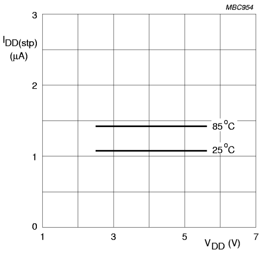
Fig.8 Typical supply current in Stop mode ( I_{DD(stp)} ) as a function of operating supply voltage ( V_{DD} ).
