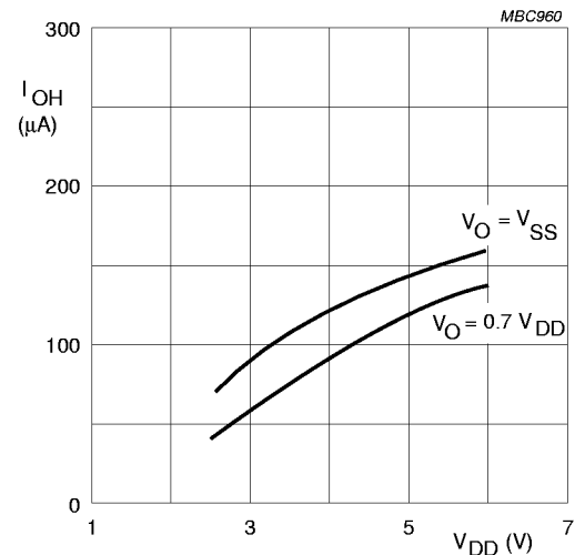
Fig.12 Typical HIGH level pull-up output source current ( I_{OH} ) as a function of operating supply voltage ( V_{DD} ).
