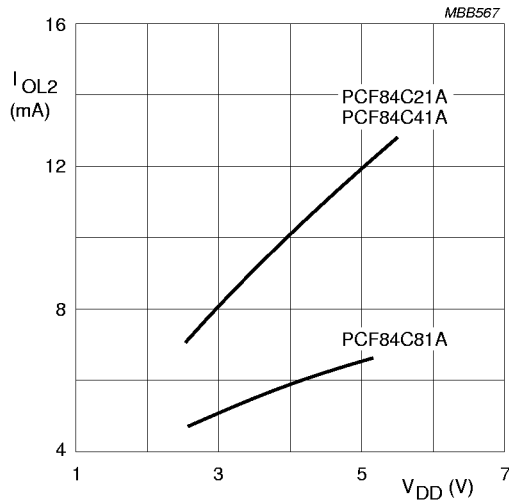
Fig.11 Typical LOW level output sink current for SDA/P2.3 or SCLK ( I_{OL2} ) as a function of operating supply voltage ( V_{DD} ).
