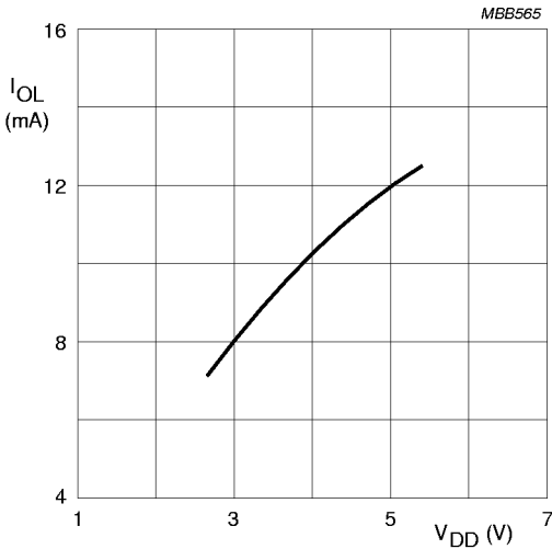
Fig.9 Typical LOW level output sink current ( I_{OL} ) as a function of operating supply voltage ( V_{DD} ).
