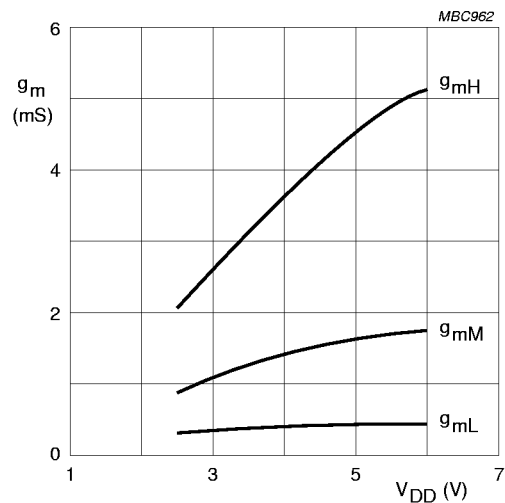
Fig.14 Typical transconductance values ( g_m ) as a function of operating supply voltage ( V_{DD} ) for the options g_{mL} , g_{mM} and g_{mH} .
