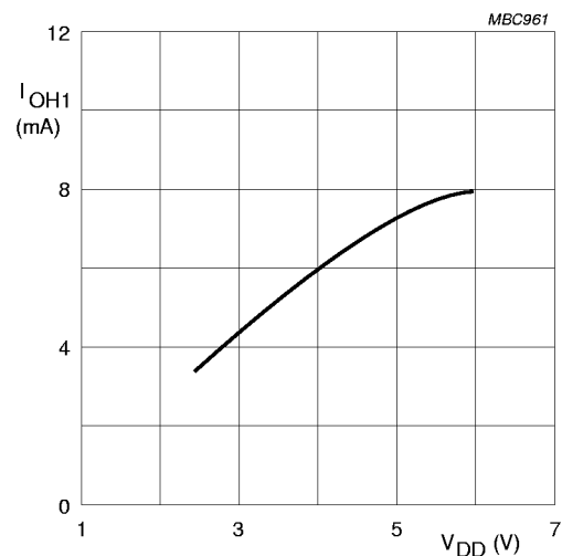
Fig.13 Typical HIGH level push-pull output source current ( I_{OH1} ) as a function of operating supply voltage ( V_{DD} ).
