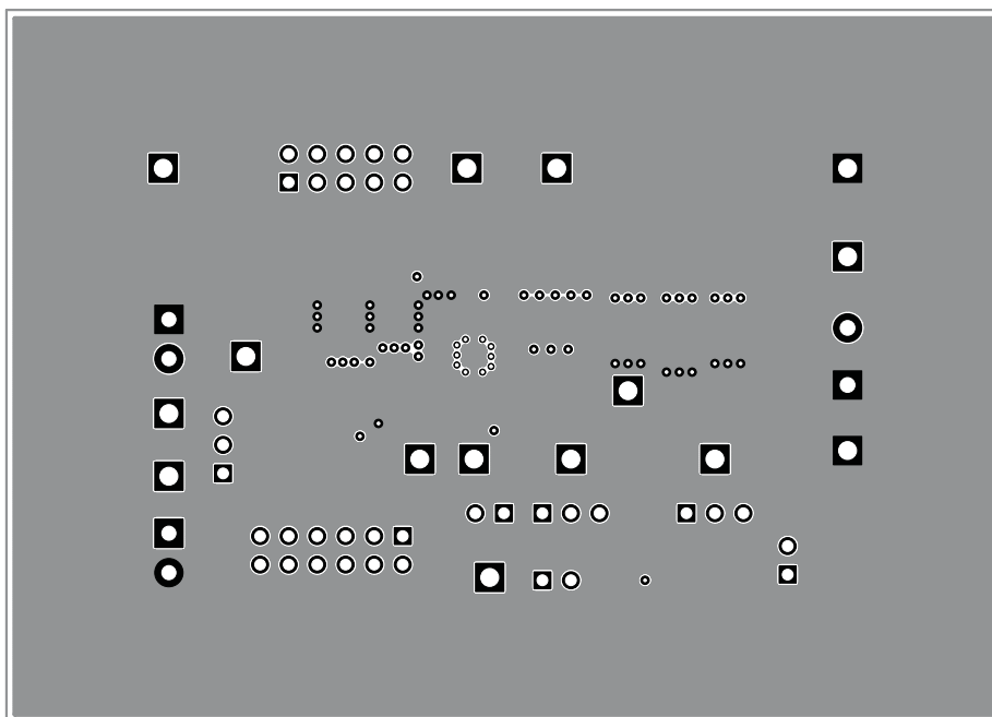
Figure 14. TPS84x2xEVM-692 Layer 2
