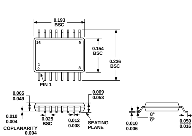
Figure 40. 16-Lead Shrink Small Outline Package [QSOP] (RQ-16)
