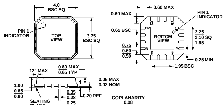
Figure 42. 16-Lead Lead Frame Chip Scale Package [LFCSP] (CP-16)
