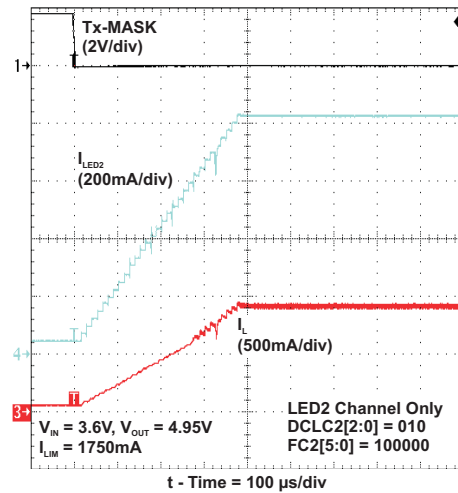
Figure 63. Tx-Masking Operation
