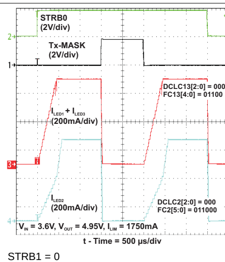
Figure 61. Tx-Masking Operation
