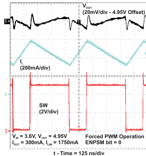
Figure 65. PWM Operation
