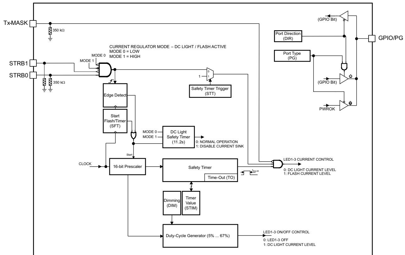
Figure 27. Timer Block
