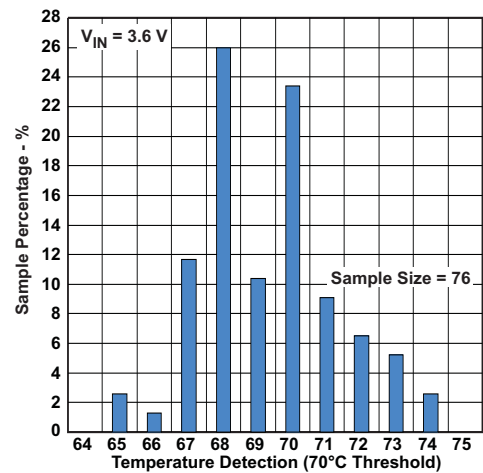
Figure 22. Temperature Detection Threshold
