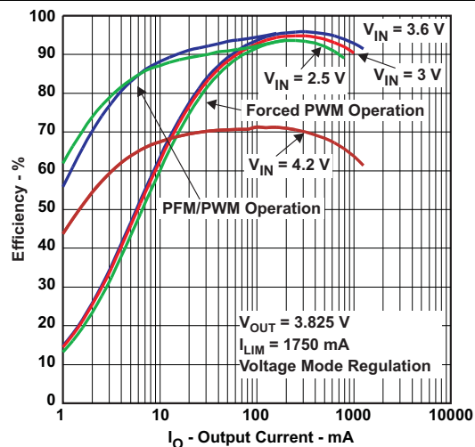
Figure 14. Efficiency vs Output Current
