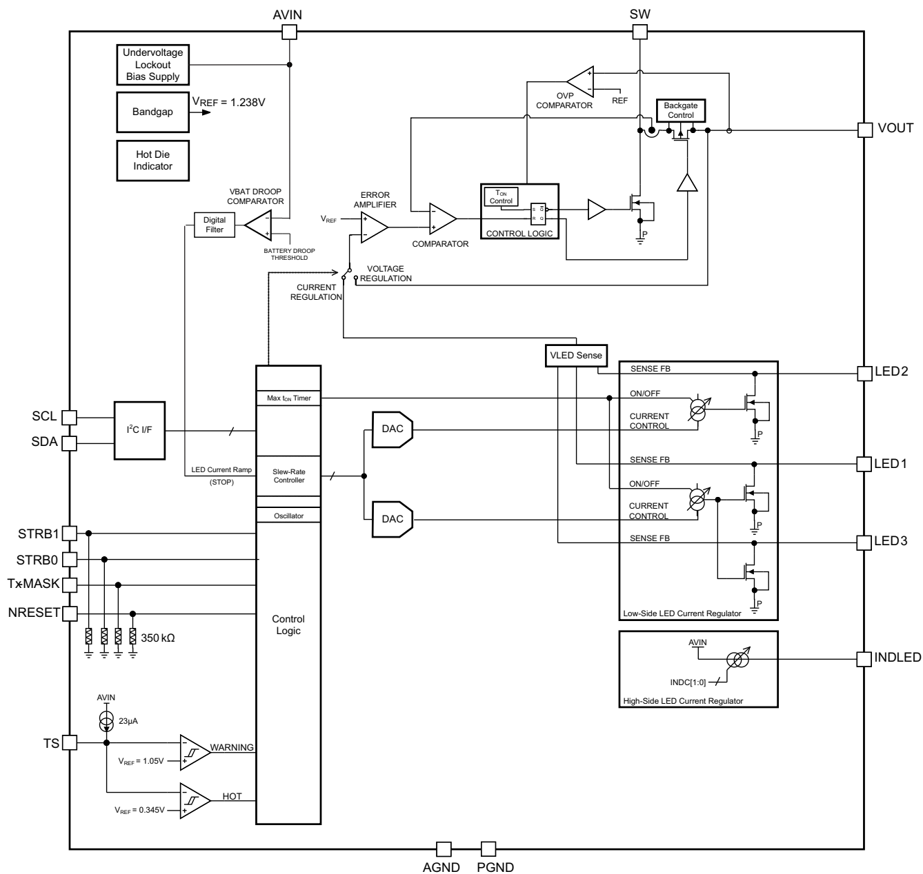
Figure 26. TPS6131x
