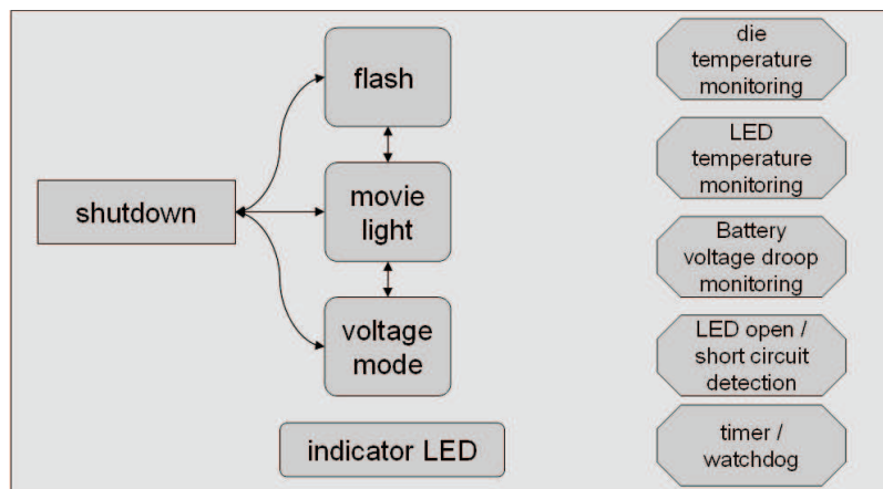
Figure 25. TPS6131x States
