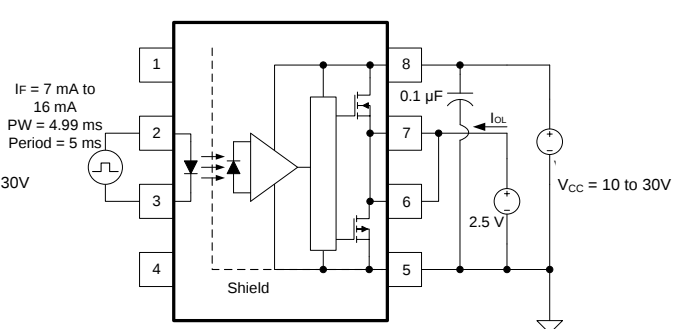
Figure 15 : V OL Test Circuit
