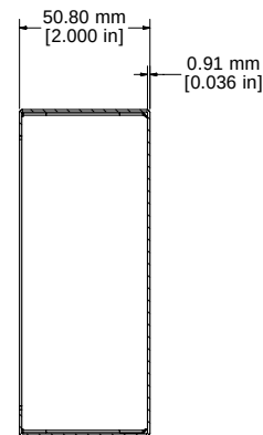
SECTION EE-EE
