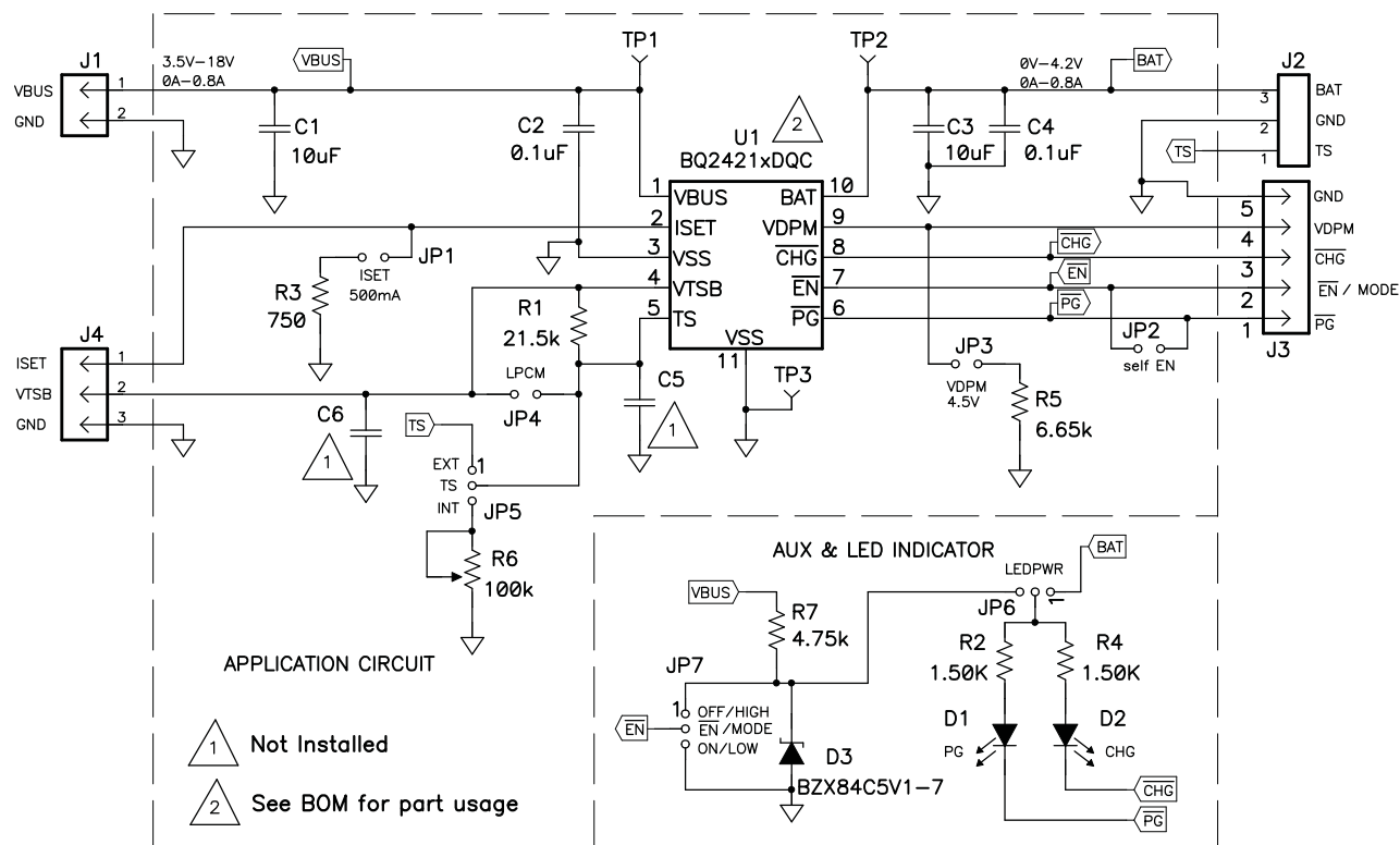
Figure 5. bq24210 EVM Schematic
