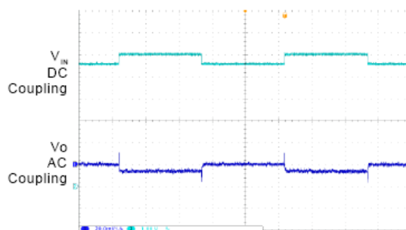
10. Line Transient
