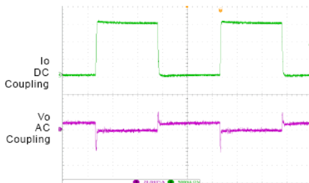
11. Load Transient
