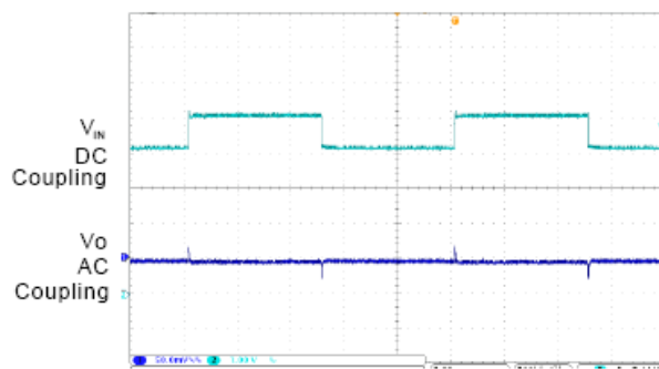
9. Line Transient
