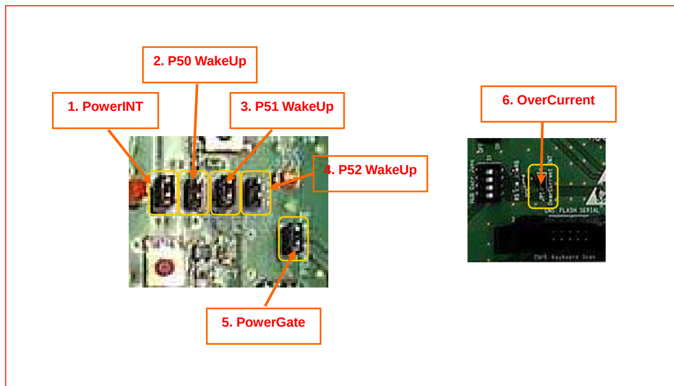
Figure 1.9 Jumper Settings
