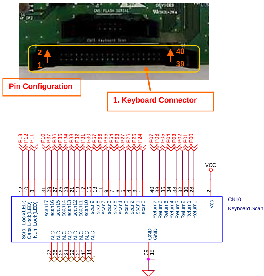
Figure 1.8 Connection Diagram for Keyboard Connector
