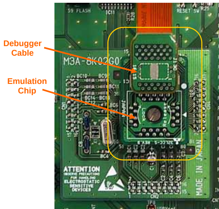
Figure 1.3(2) G02 and Debugger Connection
