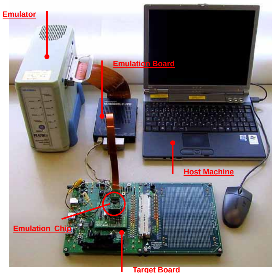
Figure 3.1 Development Environment Example
