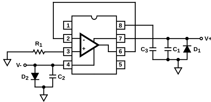
HA7-2510/883 Cerdip
